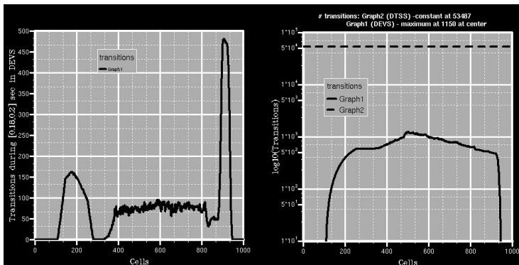
Fig. 6. The number of state changes computed by the DEVS simulator during the time interval [0, 0.18, 0.2] (left) and [0, 0, 0.2] (right).
