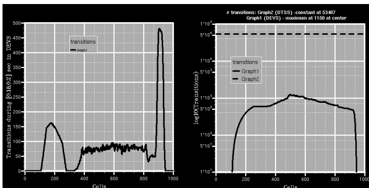
Fig. 6. The number of state changes computed by the DEVS simulator during the time interval [0.18, 0.2] (left) and [0.0, 0.2] (right).
